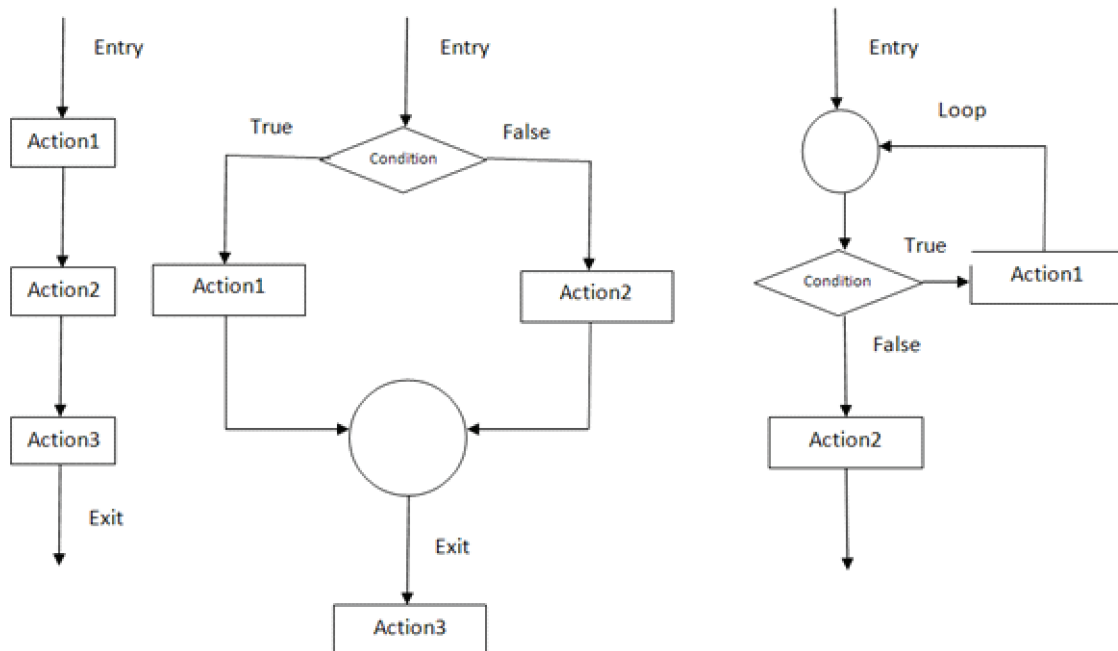
Fig. 3.4 Basic control structures
