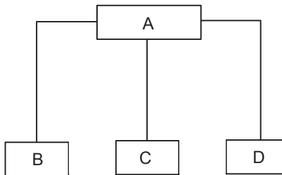
Hierarchical Inheritance
