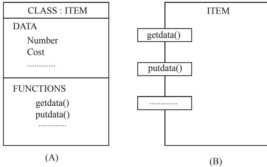
Fig. 5.2 Representation of a class
