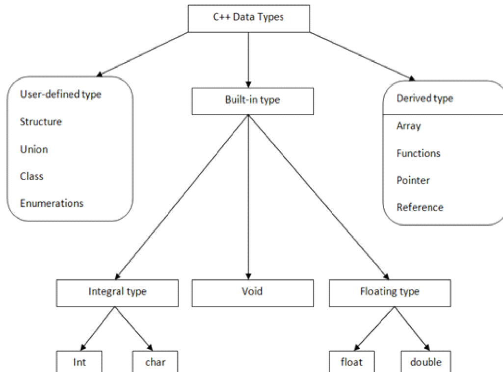
Fig 3.5 Hierarchy of C++ data types
