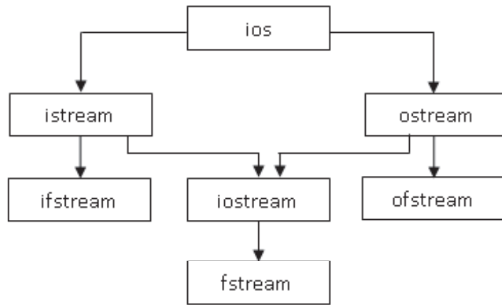
Fig 12.2 Stream class hierarchy
