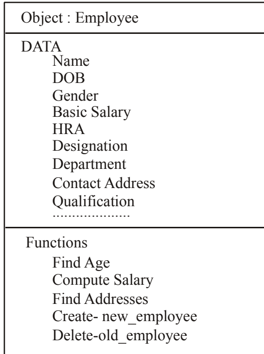
Representing of object
