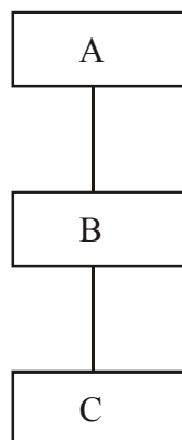
Multilevel inheritance
