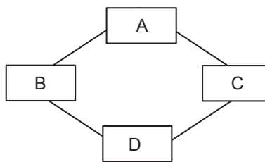
Hybrid Inheritance
