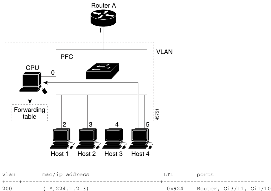
Figure 15-2 Second Host Joining a Multicast Group
