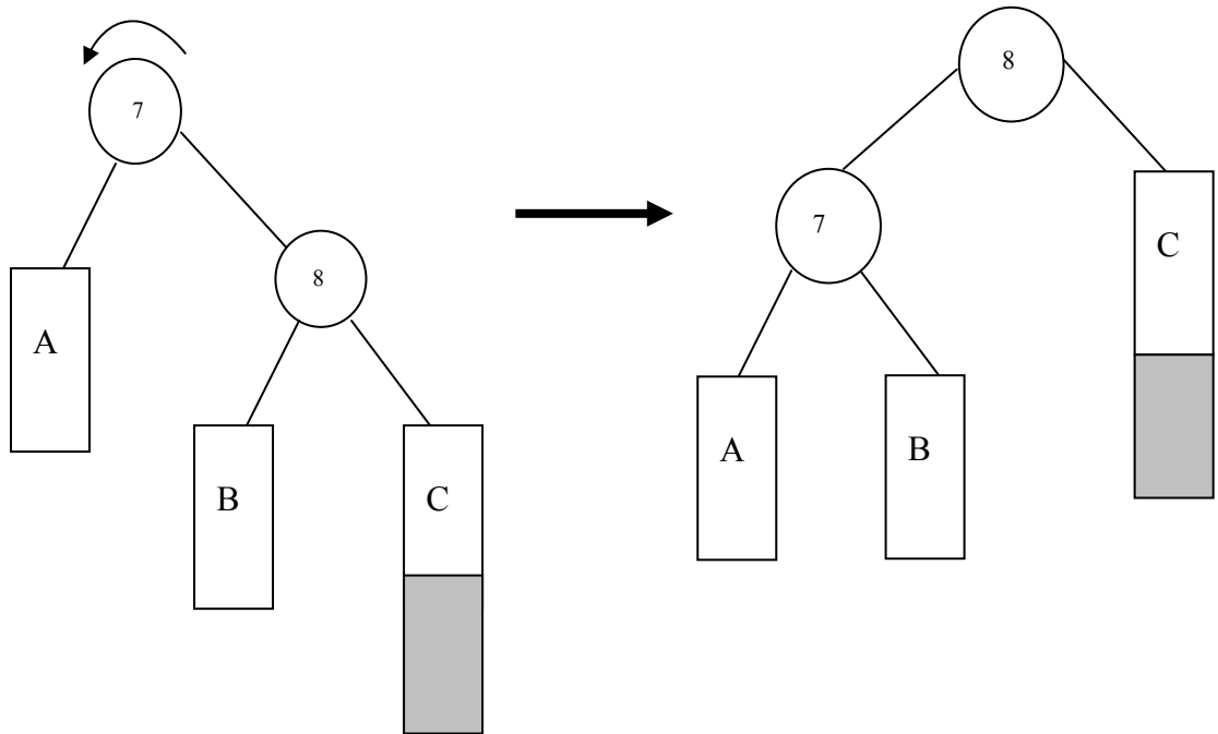
Figure 7.9: LL Rotation
