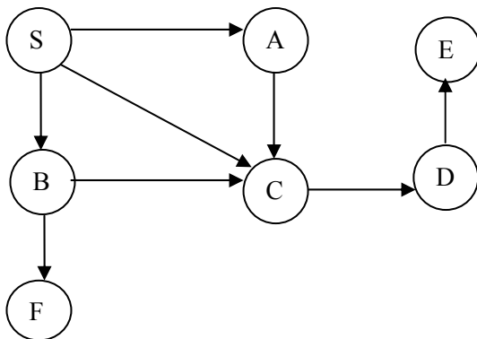
Figure 8.13 : A Digraph
