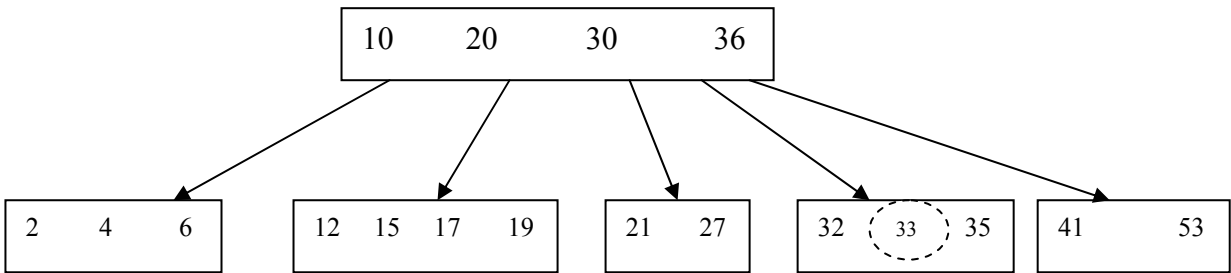
Figure 7.12 : A B-tree
