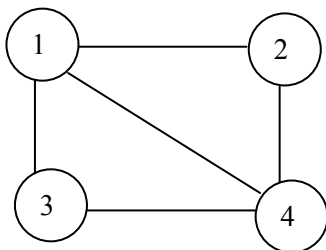
Figure 8.4: A Graph
