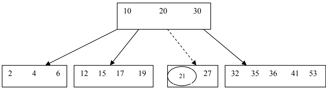
Figure 7.13 : A B-tree
